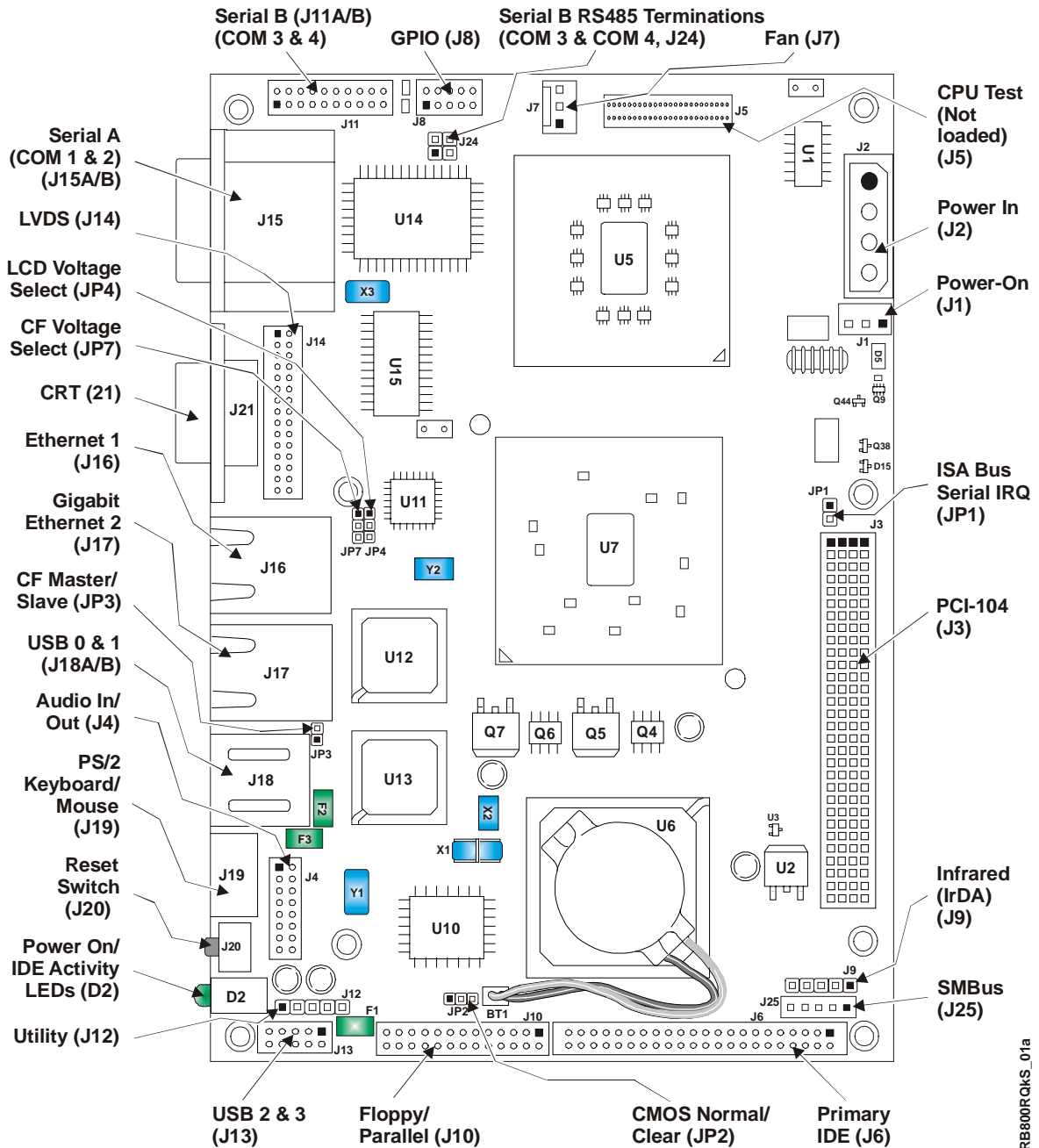
Figure 1-4. ReadyBoard 800 Connector and Pin-Locations
