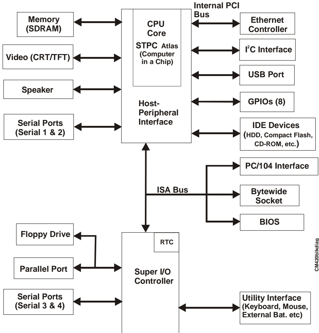
Figure 2-2. Block Diagram
