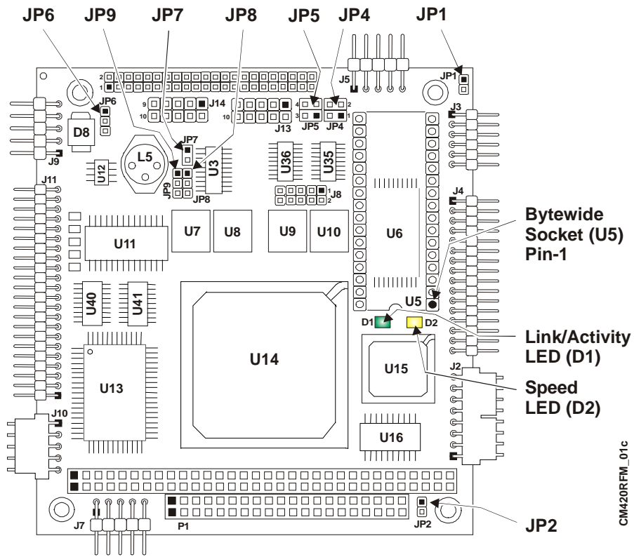
Figure 2-5. Jumper and LED Locations (Top View)
