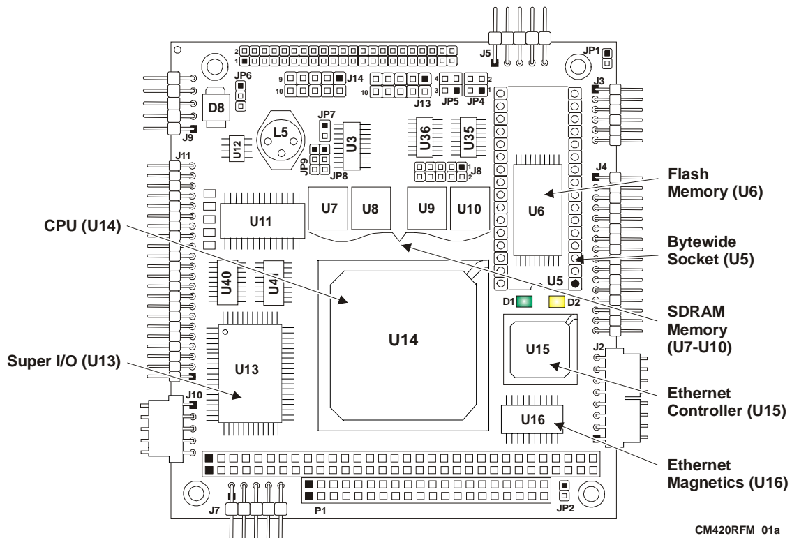
Figure 2-3. Component Locations (Top View)
