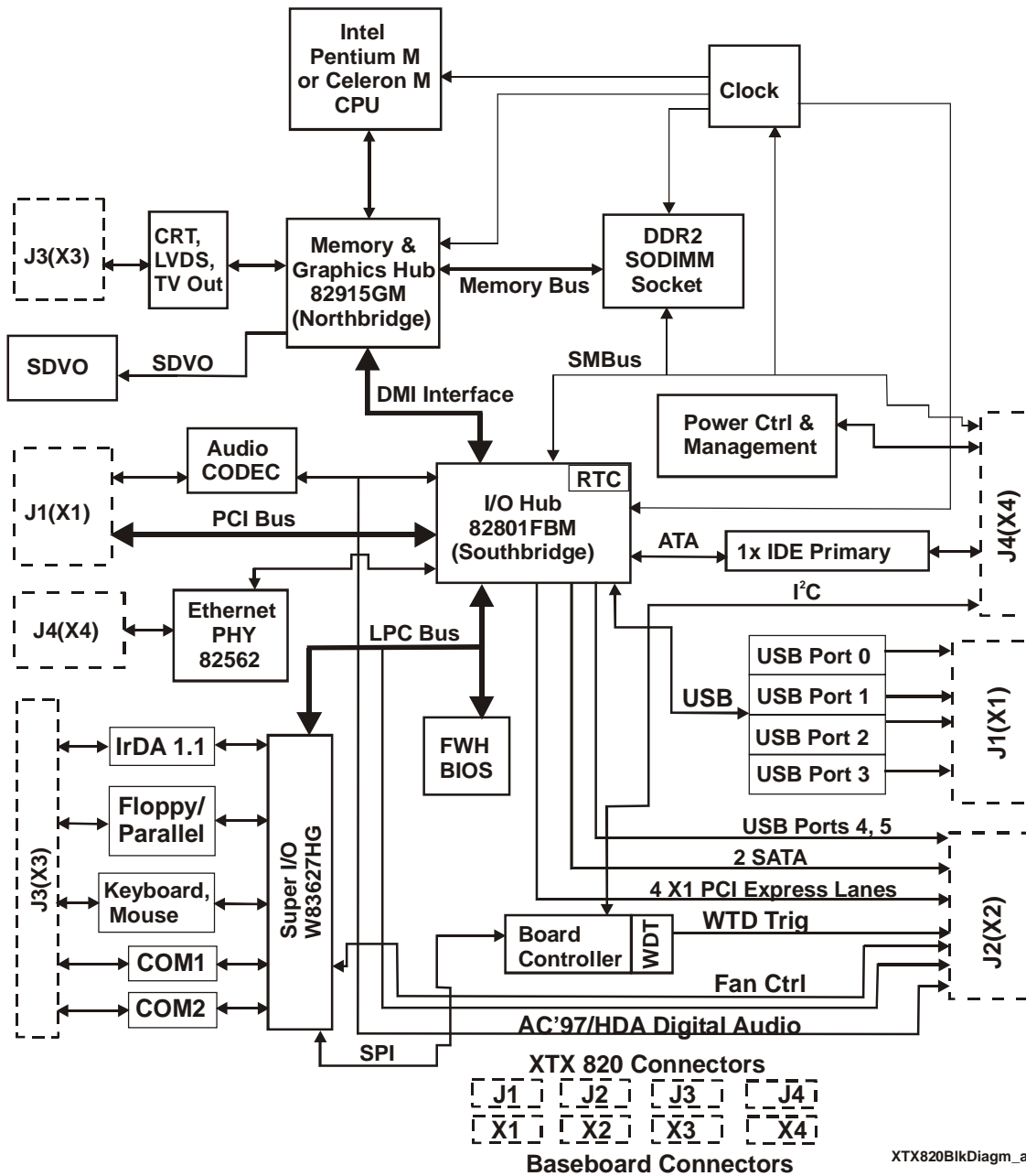
Figure 2-3. Functional Block Diagram
